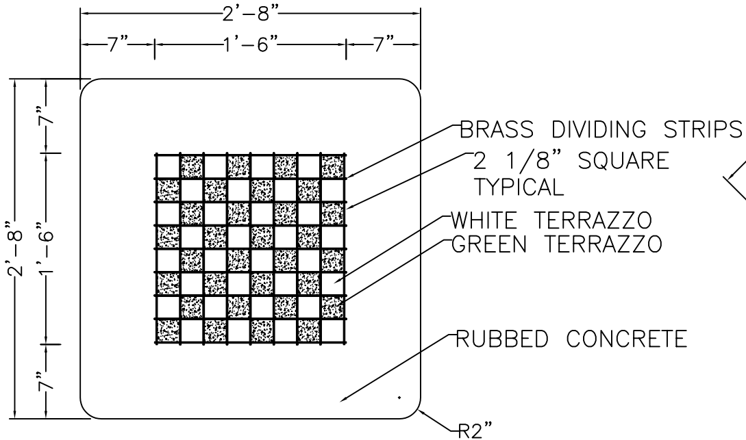
PLAN VIEW
